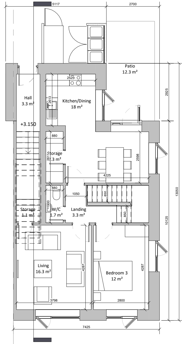
② First Floor Plan (Duplex 3A2 & 3B2) 1 : 100
