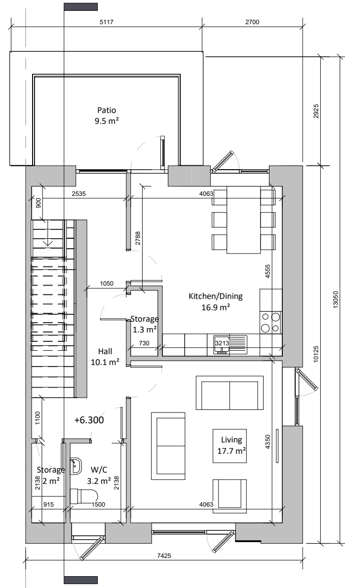
③ Second Floor Plan (Duplex 3B2) 1 : 100
