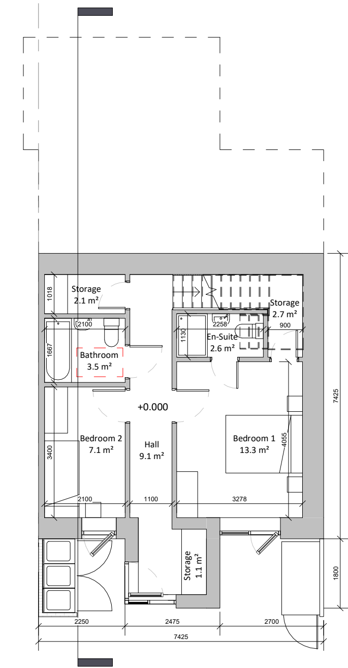
① Ground Floor Plan (Duplex 3A2) 1 : 100
