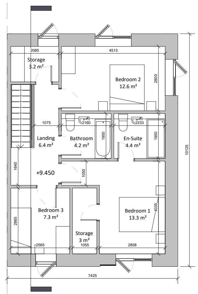
④ Third Floor Plan (Duplex 3B2) 1 : 100
